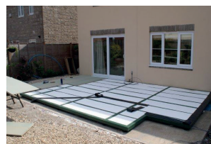
Insulation sheets fitted in to steel sections
