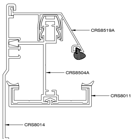
GABLE RAFTER ASSEMBLY
