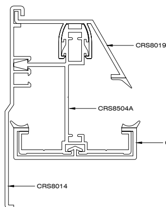
GABLE RAFTER ASSEMBLY
